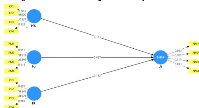
Figure 1. PLS-SEM Algorithm Output Model Results
