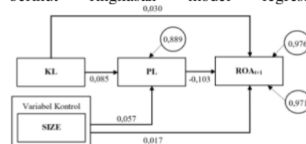
Gambar 1. Model Regresi
